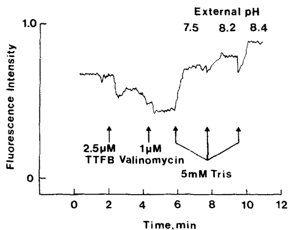
Fig.2. \text{pH}_i Calibration of quene 1 in a single mouse thymocyte. The relative fluorescence intensity (F.I.) of about 0.4 mM quene 1 in a mouse thymocyte in 3 ml of high \text{K}^+ medium (103 mM \text{KCl} , 5.6 mM \text{NaCl} , 10 mM HEPES, 0.42 mM \text{CaCl}_2 , 0.41 mM \text{MgCl}_2 , pH 7.2. Additions of TTFB (7.5 \mu\text{l} of 1 mM in ethanol), 1 \mu\text{M} valinomycin (3 \mu\text{l} of 1 mM in DMSO) and 5 mM Tris (15 \mu\text{l} of 1 M Tris in PBS) were made as shown. (1.0 F.I. = 4 \times 10^5 photon cps, and corresponds to about the maximal fluorescence of quene 1 as in fig.1.)
