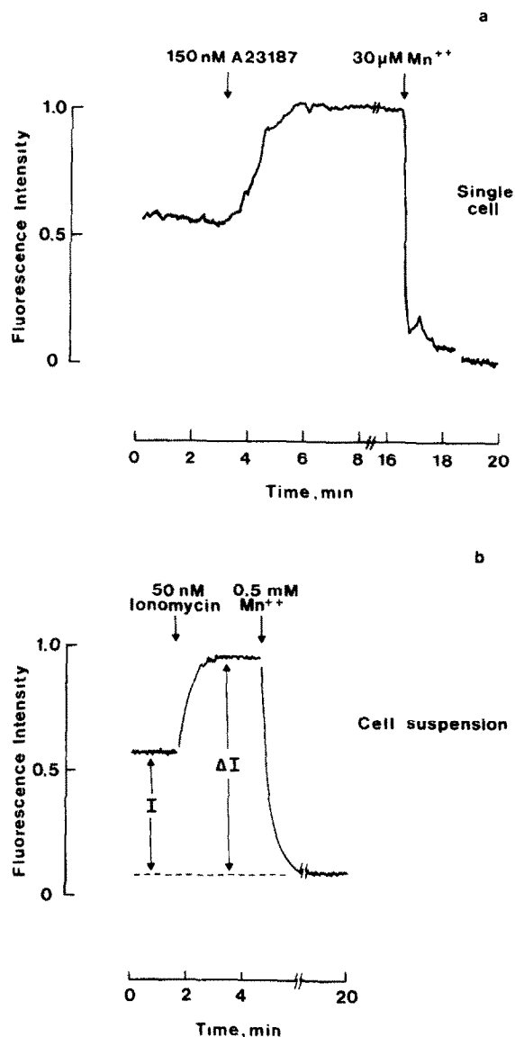
Fig.3. [\text{Ca}]_i Calibration of quin 2 in a single mouse thymocyte. (a) Relative fluorescence intensity of a mouse thymocyte loaded with about 2 mM quin 2 and treated with 150 nM A23187 (3 \mu\text{l} of 150 \mu\text{M} A23187 in DMSO) followed by 30 \mu\text{M} \text{MnCl}_2 (9 \mu\text{l} of 10 mM \text{MnCl}_2 ). 1.0 F.I. = 10^5 photon cps. The percentage saturation of \text{Ca} -quin 2 was calculated from:
